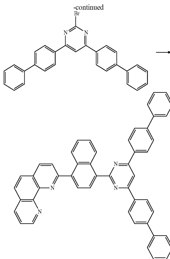
[Reaction Formula 6-2]
