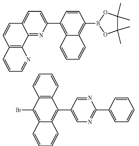
[Reaction Formula 8]
