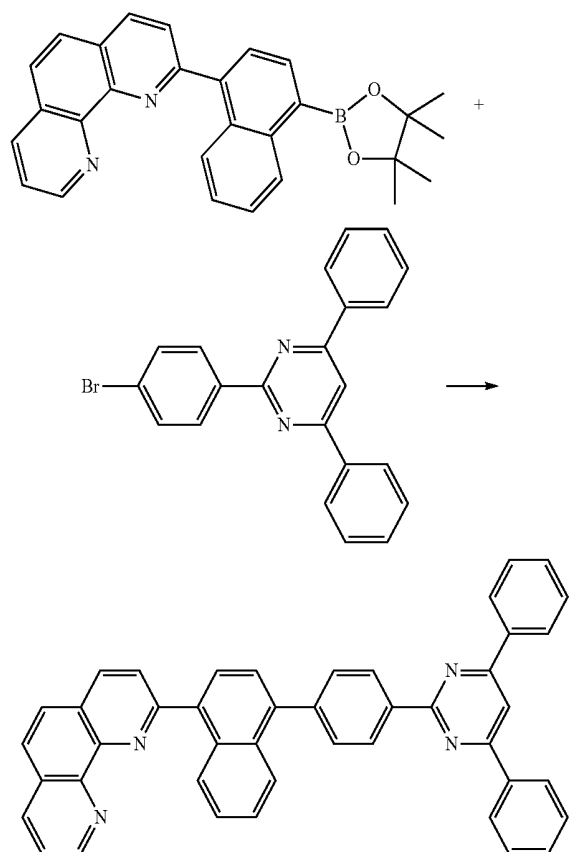
[Reaction Formula 6-2]
