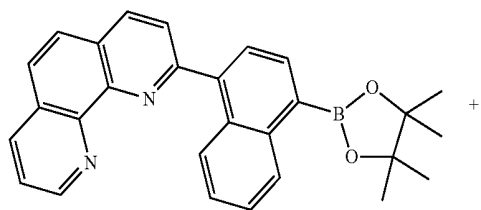
[Reaction Formula 7]
