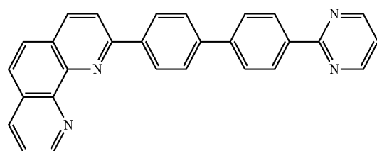
[Formula 2]
